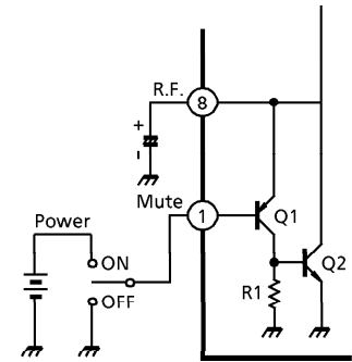
Fig.5 Mute circuit
